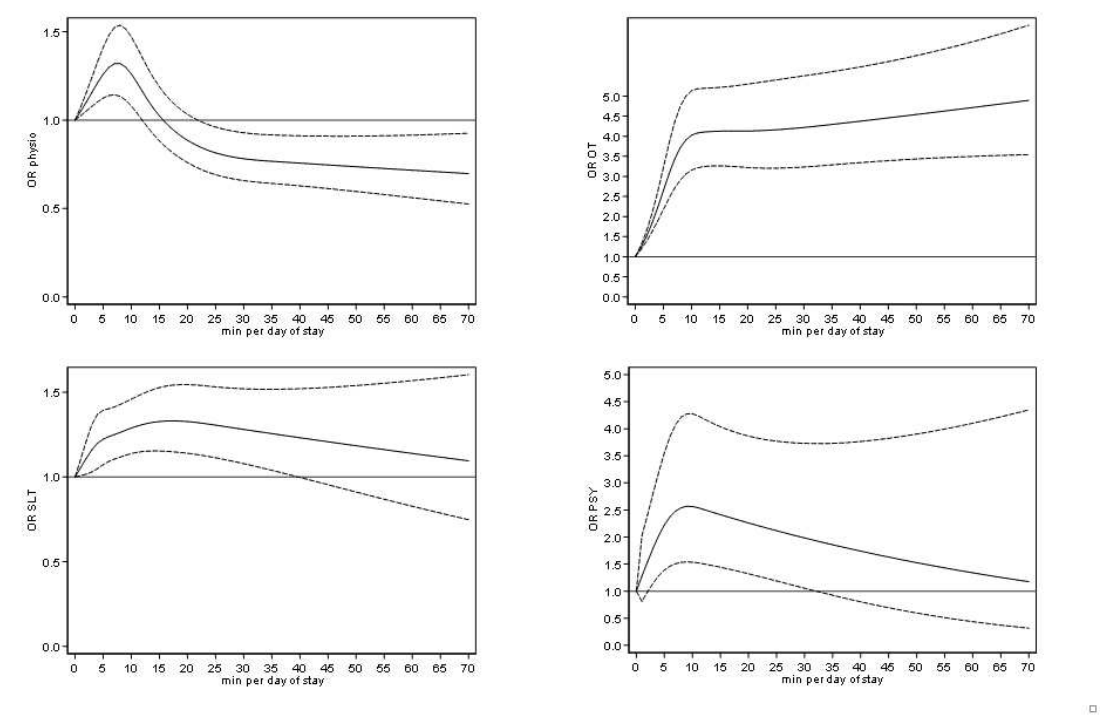
Supplementary Figure 2. Cubic Splines Plot of the Odds Ratio (95% CI) for Home on discharge per minute of therapy / inpatient day of stay (referenced to zero) – As produced from the fully adjusted multilevel mixed effects regression model
