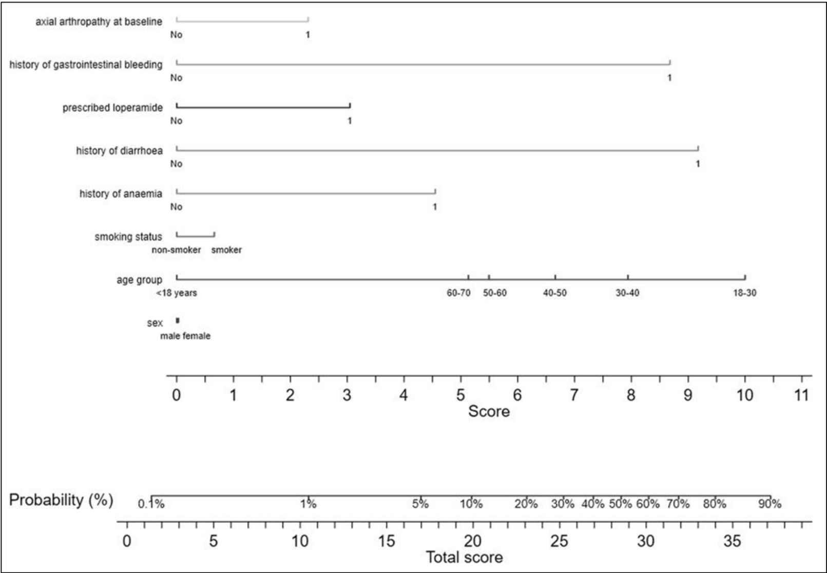
Appendix 7: Nomogram: prediction of inflammatory bowel disease diagnosis within 3-years of a diagnosis of anterior uveitis
