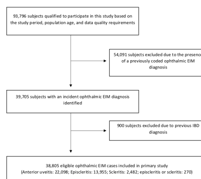
Figure 1 Study flow chart. EIM, extraintestinal manifestation; IBD, inflammatory bowel disease.
