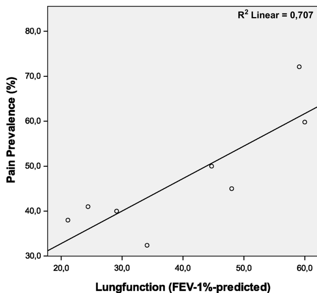
Figure 5 Relationship between lungfunction and pain prevalence. Each data point represents a separate study. Correlation coefficient: Spearmans r=0.79 ( p=0.021 ).
