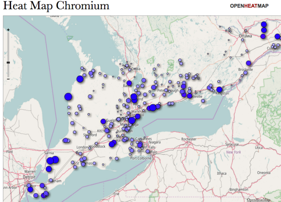
Figure 7 Heat map showing the concentration of chromium in 2014 in various streams around Southwestern Ontario. Map created using 2014 data from the Provincial (Stream) Water Quality Monitoring Network at https://www.ontario.ca/data/provincial-stream-water-quality-monitoring-network in open-source software found at www.openheatmap.com .
